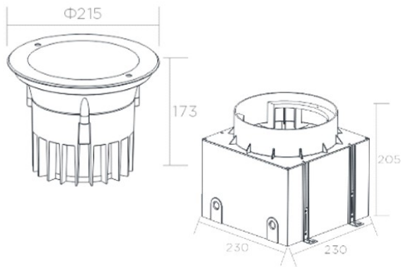
Sizes drawing
